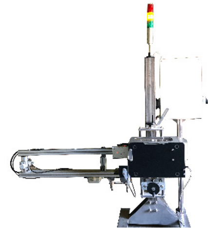
N-PR-03 Label Printer Applicator
