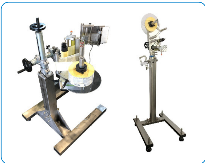
Automatic label applicator A 150
